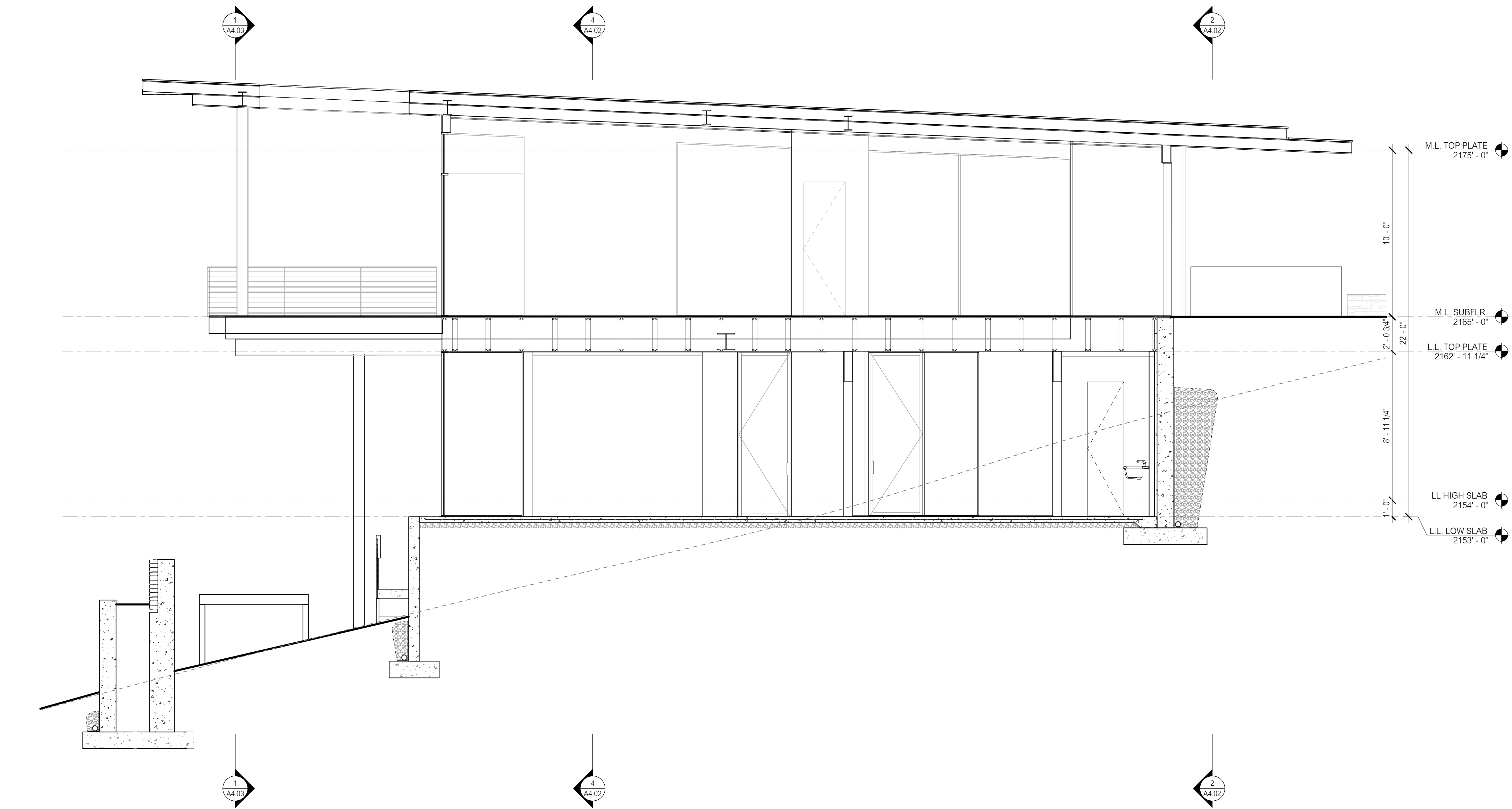
2 N-S SECTION - DINING AND FOYER 1/4" = 1'-0"
