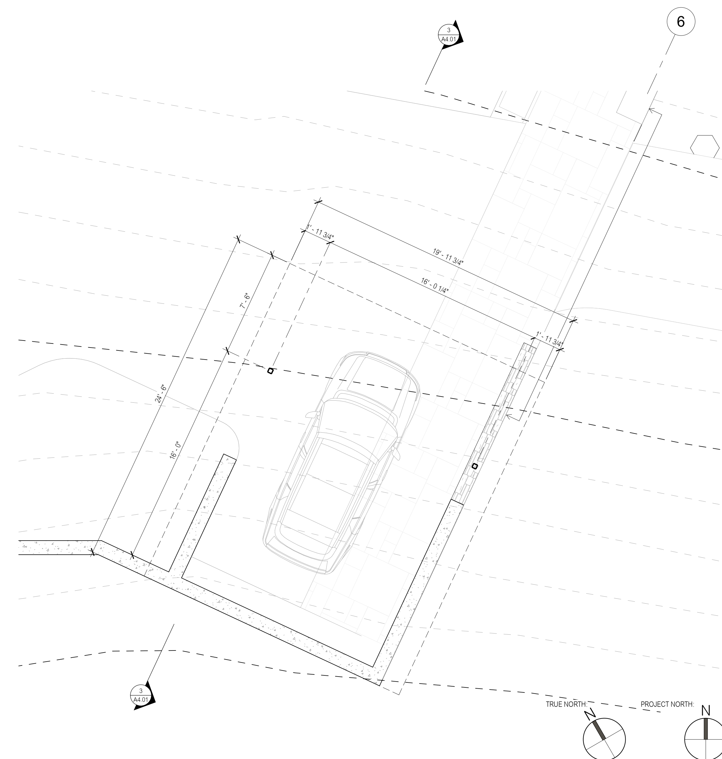
1 CARPORT - FLOOR PLAN 1/4" = 1'-0"
