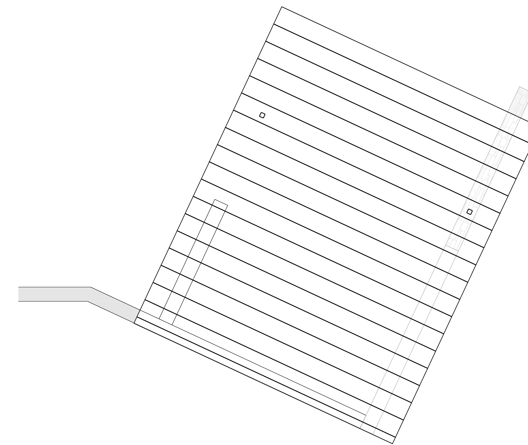
3 CARPORT - FRAMING PLAN 1/4" = 1'-0"
